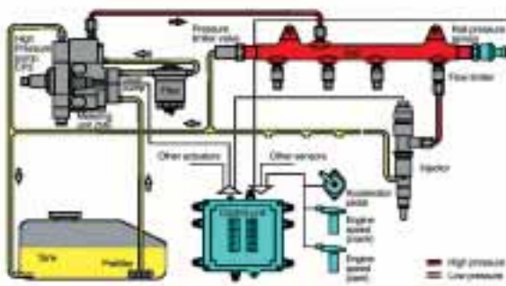
“Common Rail” Doosan DLo6 Engine
